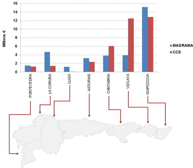
Figure 6.- Spatial pattern of economic losses (Public Insurance Office (CCS) and Spanish Coastal Authority (MAGRAMA))
