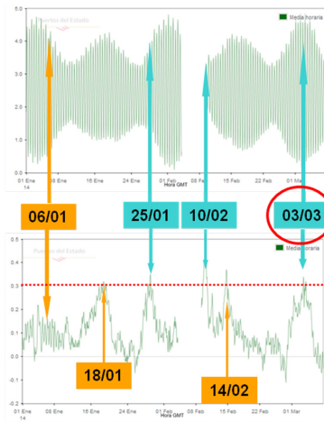
Figure 3: Sea level (upper panel) and non tidal residuals (surges, lower panel) measured in the tide gauge of Bilbao from January 1 st to March 5 th .
