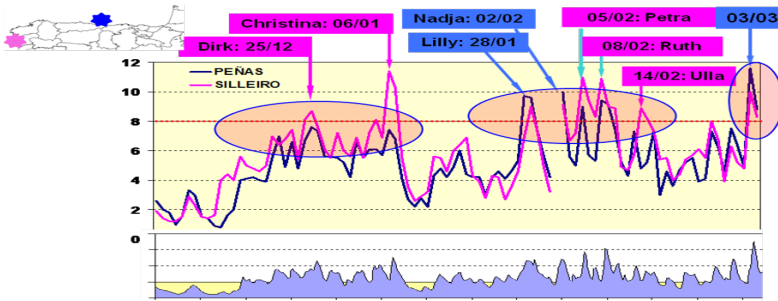
Figure 1: Maximum daily Significant Wave height from two buoys from December 1st 2013 to March 5th 2014. The 8 m SWH equals the long-term daily 95th percentile.
