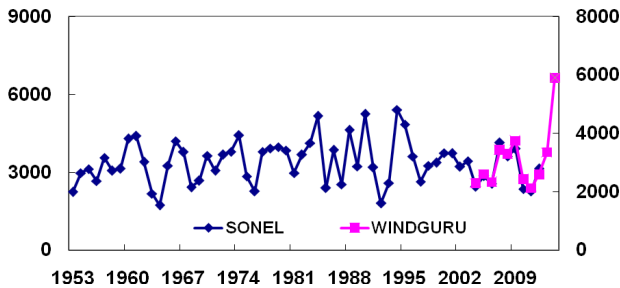
Figure 2: Wave energy evolution from two wave models ( http://www.sonel.org/ and http://www.windguru.cz/ ).
