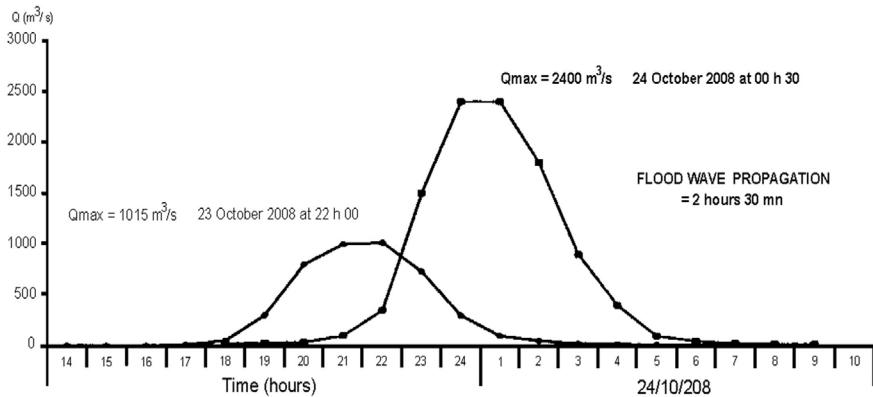
Figure 5. Oued Kert flood hydrograph.
