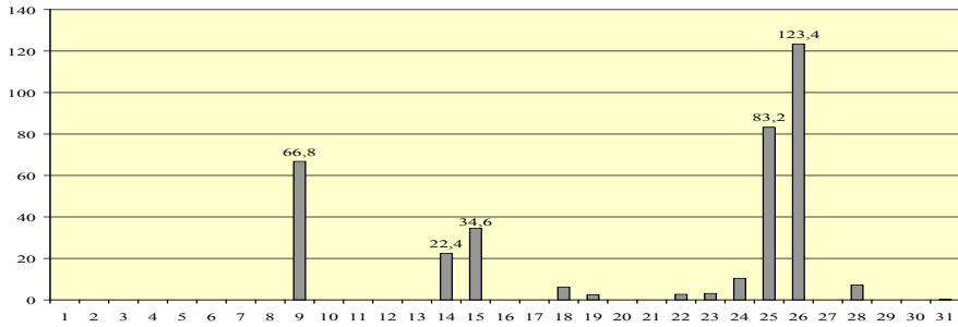
Figure 4. Rainfall in October 2008.
