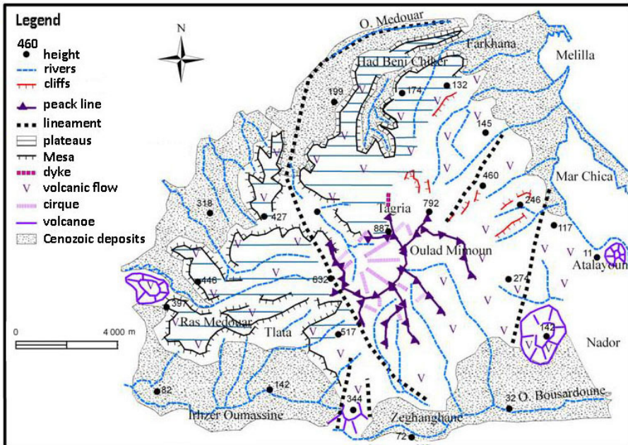
Figure 2. The main geomorphologic units of the massif of Gourougou.
